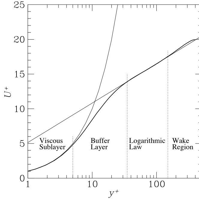
FIGURE 4. Mean velocity profile for the channel flow. The logarithmic-law region is fitted by the equation U^+ = 5.136 + 0.4053^{-1} \ln y^+ .
