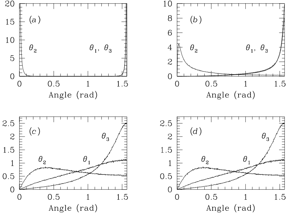
FIGURE 12. Probability density function (PDF) estimates for the angle made between the vorticity and the principal strain rate directions. (a) viscous sublayer, (b) buffer layer, (c) log-law region, (d) wake region.
