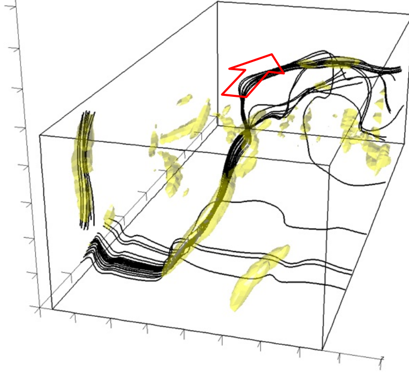
FIGURE 10. Structures with stable focus/stretching topology (shaded yellow) showing vortex lines which run through selected cores. Box size in wall units: \Delta x^+ = 590 , \Delta y^+ = 190 and \Delta z^+ = 285 .
