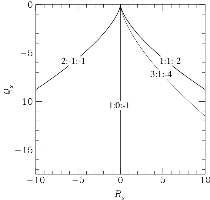
FIGURE 3. Lines in (Q_s, R_s) space corresponding to different ratios of principal strains \lambda_1:\lambda_2:\lambda_3 . All (Q_s, R_s) pairs must fall below the lines corresponding to the ratios 2:-1:-1 and 1:1:-2 as a consequence of the symmetry of \mathbf{S} .
