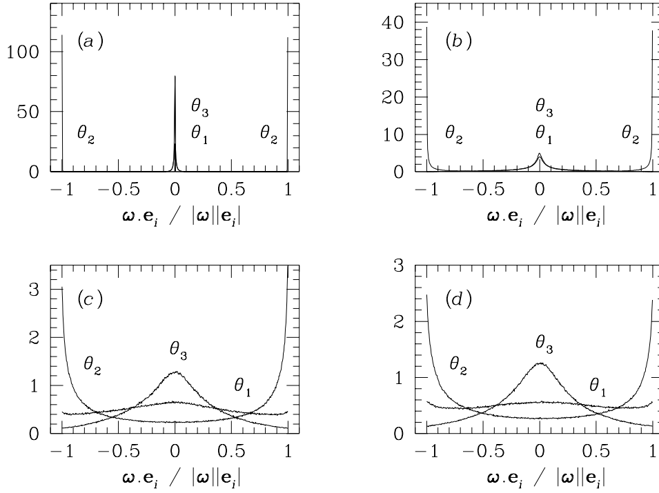
FIGURE 13. Probability density function (PDF) estimates for the cosine of the angle made between the vorticity and the principal strain rate directions. (a); viscous sub-layer, (b); buffer layer, (c); log-law region, (d); wake region.
