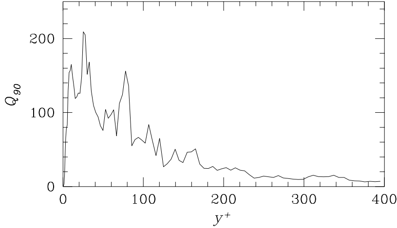
FIGURE 7. Plot of the 90th percentile of Q as a function of y^+ from one realization of the flow. Velocity gradients have been normalized by \overline{U}_c/\delta .
