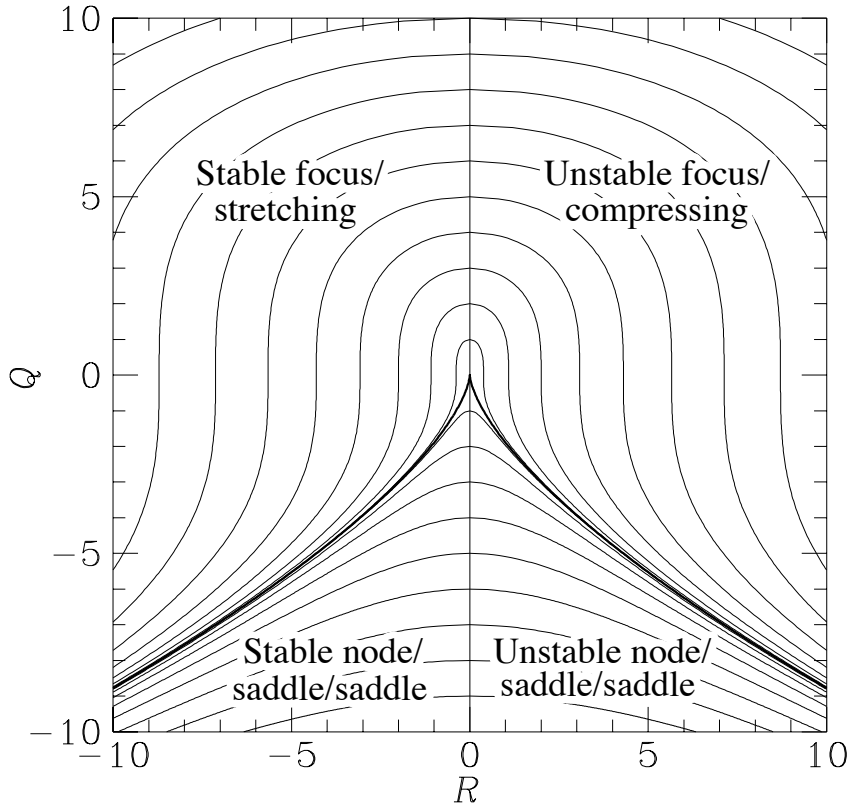
FIGURE 1. Plot showing the space of tensor invariants Q and R for incompressible flow, with lines corresponding to constant values of the discriminant D = (27/4)R^2 + Q^3 . The different regions are labelled according to the terminology of Chong et al. (1990).
