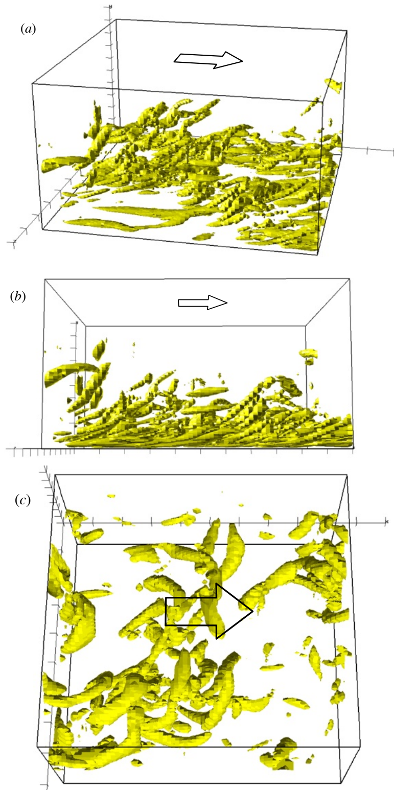
FIGURE 9. View of structures with stable focus/stretching topologies shown in figure 8(c), looking: (a) from above and downstream, (b) spanwise along the wall, (c) from above (this last view shows only structures in the outer regions of the flow, using a lower contouring level than in a and b ).
