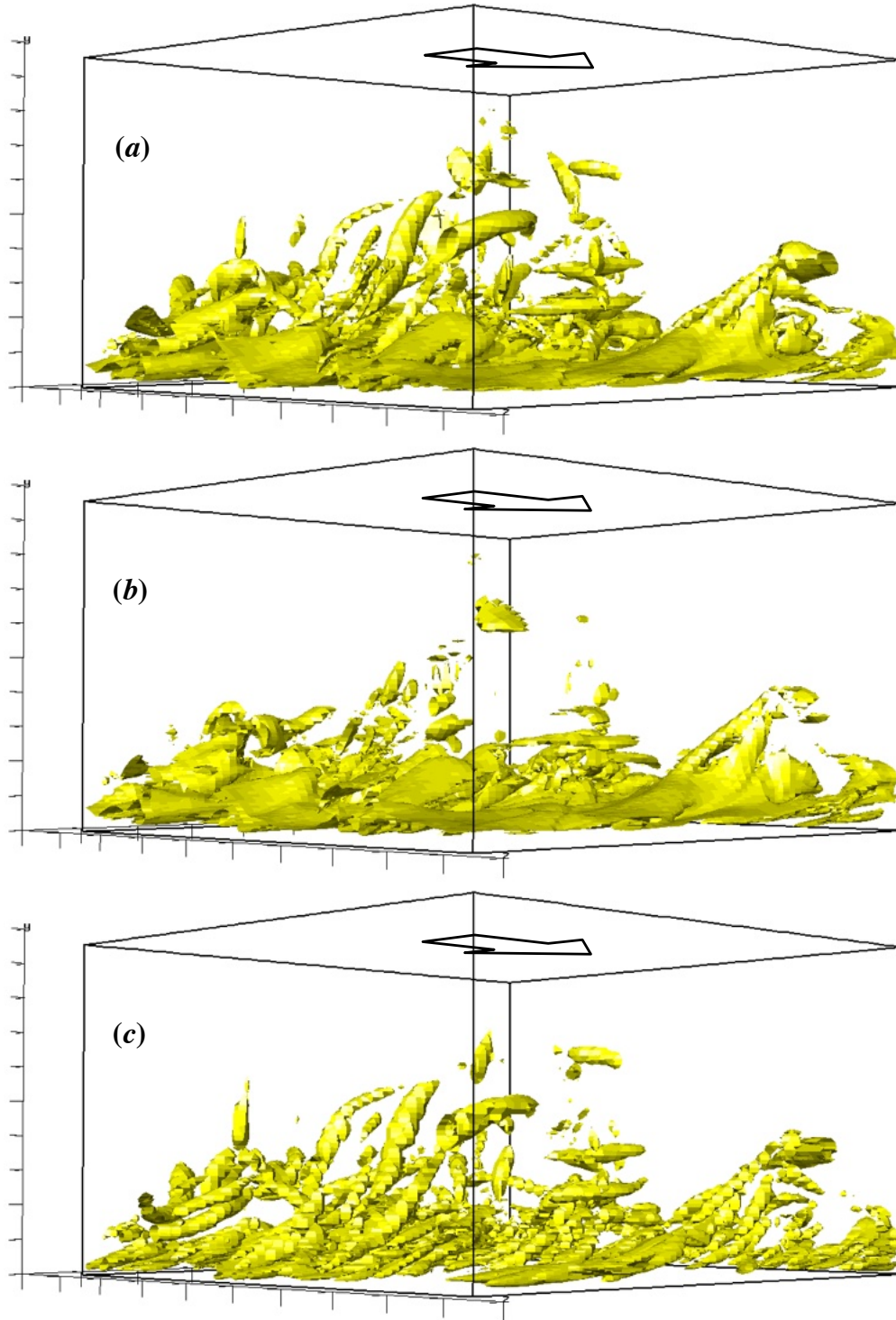
FIGURE 8. Flow visualization in subset of the flow bounded below by the wall. (a) iso-surfaces of enstrophy -\Omega_{ij}\Omega_{ji} , (b) iso-surfaces of viscous dissipation (proportional to S_{ij}S_{ji} ), (c) iso-surfaces of discriminant D (for R \leq 0 : intensity of stable focus/stretching topology). Box size in wall units: \Delta x^+ = 670 , \Delta y^+ = 375 and \Delta z^+ = 640 . Mean flow direction indicated by arrows.
