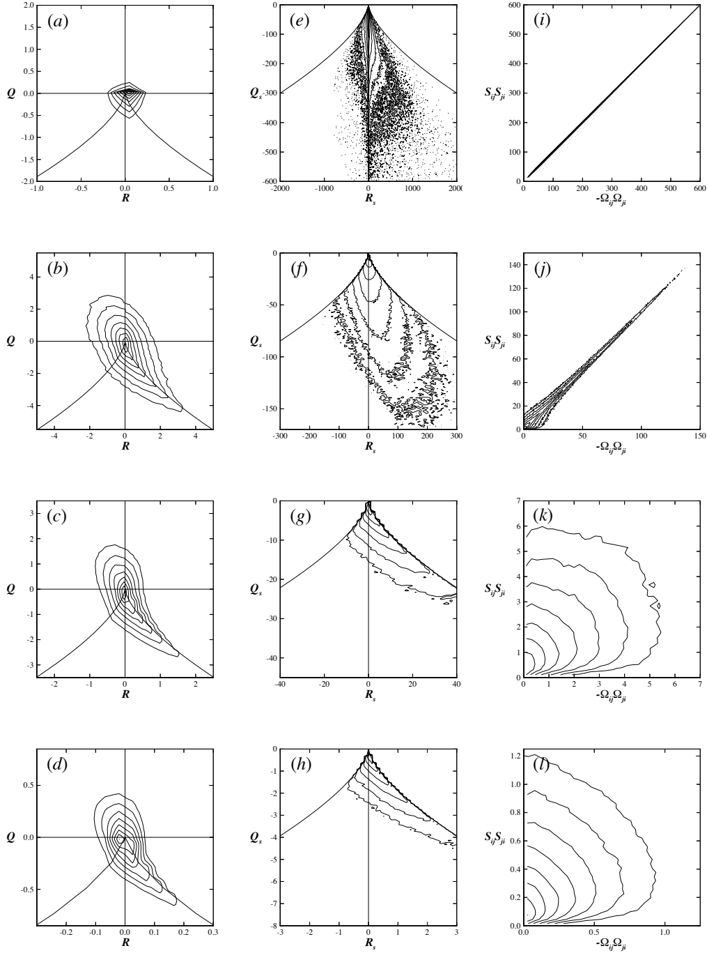
FIGURE 6. PDF plots of (a–d); Q vs. R , (e–h); Q_s vs. R_s , (i–l); S_{ij}S_{ji} vs. -\Omega_{ij}\Omega_{ji} in the four flow regions: viscous sub-layer (a, e, i), buffer layer (b, f, j), log-law region (c, g, k), wake region (d, h, l). The plots show half-decade contours of relative frequency over a four-decade range. In the plots of Q vs. R and Q_s vs. R_s , the line D = (27/4)R^2 + Q^3 = 0 which divides the plane into regions where the tensor has purely real and complex-conjugate pair/real eigenvalues is shown as reference. Velocity gradients have been normalized by \bar{U}_c/\delta .
